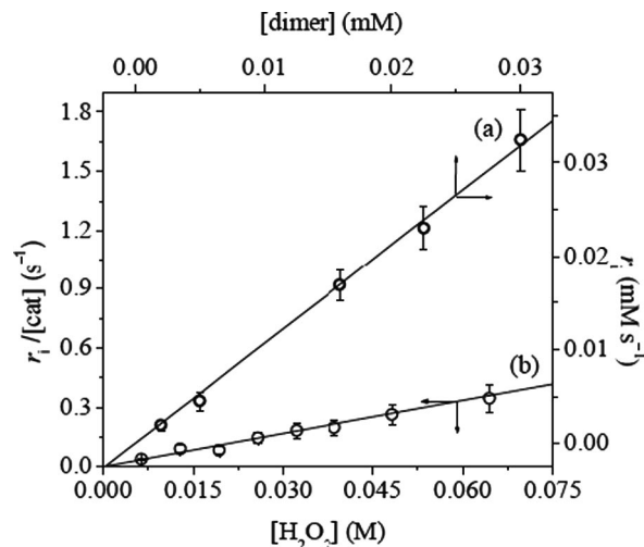
Figure 10. Effect of (a) [catalyst] ( [\text{H}_2\text{O}_2]_0 = 12.9 \text{ mM} ) and (b) [\text{H}_2\text{O}_2] on the initial rate of \text{H}_2\text{O}_2 disproportionation at 25^\circ\text{C} in dmf.
