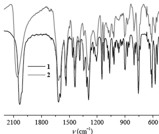
Figure 4. FTIR spectra of complexes 1 and 2 .
