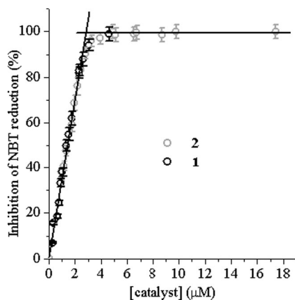
Figure 8. SOD activity of complexes 1 and 2 in the riboflavin-methionine-NBT assay.
