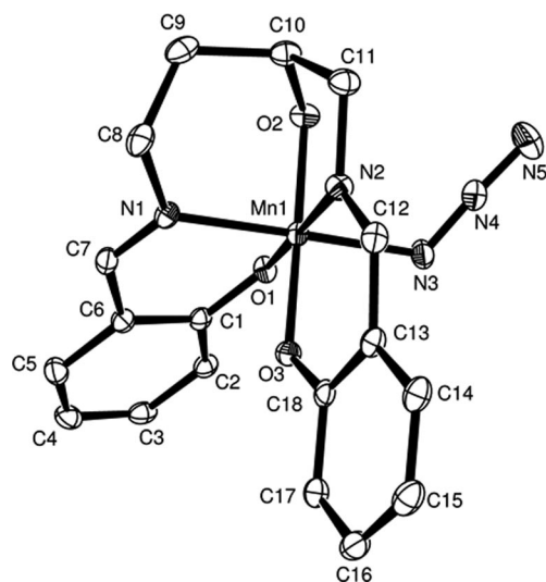
Figure 1. Plot of the asymmetric unit of [Mn(salbutO)N 3 ] ( 1 ) at the 30% probability level with atom numbering. Hydrogen atoms have been omitted for clarity. Selected bond lengths (Å) and angles (°): Mn1–N1 2.008(2), Mn1–N2 1.983(2), Mn1–N3 1.991(2), Mn1–O1 1.8619(17), Mn1–O2 1.8482(18), Mn1–O3 1.8926(18), N1–Mn1–N3 178.24(10), N2–Mn1–O1 177.53(8), O3–Mn1–O2 171.94(8), N1–Mn1–N2 92.28(9), N3–Mn1–N2 89.43(10), N1–Mn1–O3 88.70(9), N3–Mn1–O3 90.85(9), N2–Mn1–O3 90.36(8), N1–Mn1–O1 88.87(8), N3–Mn1–O1 89.44(9), O3–Mn1–O1 91.86(8), N1–Mn1–O2 88.54(9), N3–Mn1–O2 92.1(1), N2–Mn1–O2 82.19(8), O1–Mn1–O2 95.65(8).
