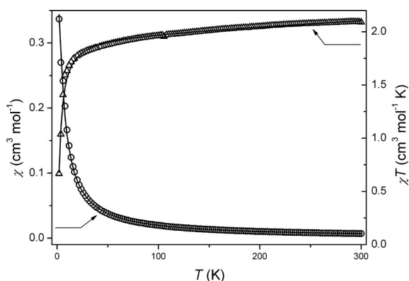
Figure 3. Temperature dependence of \chi_{\text{M}} (○) and \chi_{\text{M}}T (Δ) for compound 2 . The solid lines show the best fit based on the Heisenberg chain model (see text).
