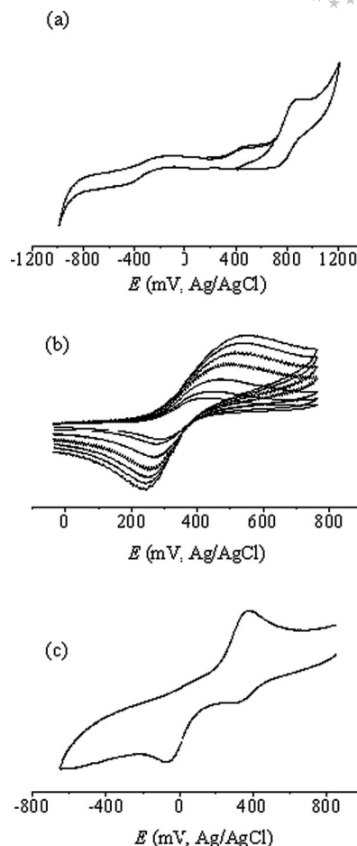
Figure 7. Cyclic voltammogram of (a) 2 in methanol, (b) 2 in dmf at various scan rates between 50 and 1000 mV, and (c) 1 in dmf a few minutes after dissolution. Conditions: Pt/Pt/Ag/AgCl; conc.: 1 mM; supporting electrolyte: Bu 4 NPF 6 . Scan rate in (a) and (c): 100 mV s –1 .
