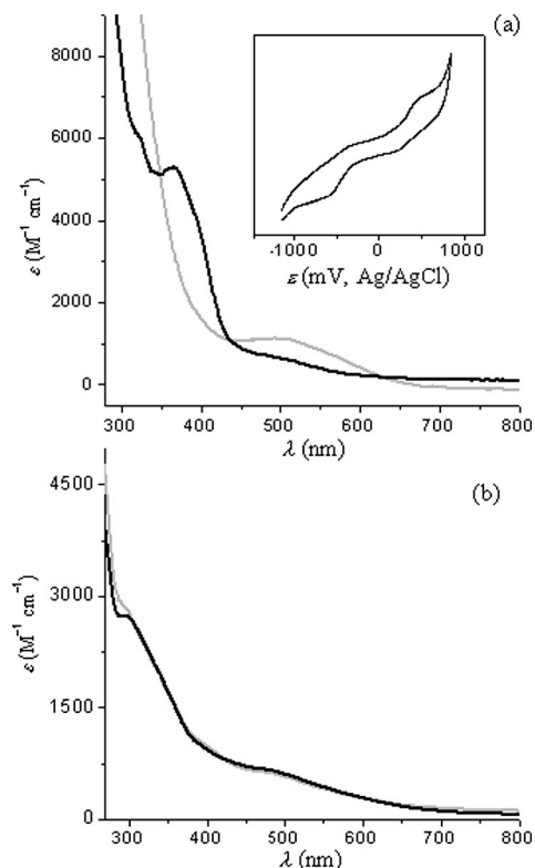
Figure 9. Electronic spectra of 2 before (black line) and after (gray line) addition of 300 equiv. of \text{H}_2\text{O}_2 , in (a) dmf (b) methanol. Inset: Cyclic voltammogram at the end of the reaction in dmf.
