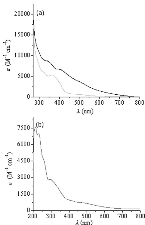
Figure 5. Electronic spectra of 1 (a) immediately (black line) and 30 min (gray line) after dissolution in dmf; (b) in methanol.
