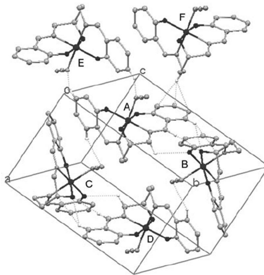
Figure 2. Crystal packing diagram for 1 , emphasizing the intermolecular hydrogen-bonding interactions.
