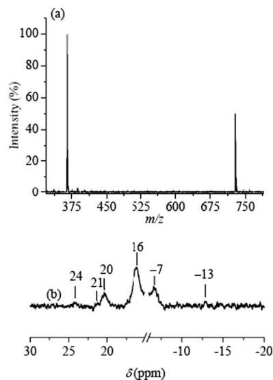
Figure 6. ESI mass spectrum of 2 in acetonitrile (a) and ^1\text{H} NMR spectrum of 2 in [\text{D}_4]\text{methanol} (ca. 10 mM) (b).
